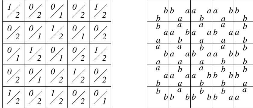
Figure 4: An up-followers diagram U and the FAC induced by it
