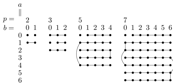
FIGURE 1. Isomorphism classes of loops \mathcal{Q}_{a,b}(\mathbb{Z}_p) for p \in \{2, 3, 5, 7\} .
