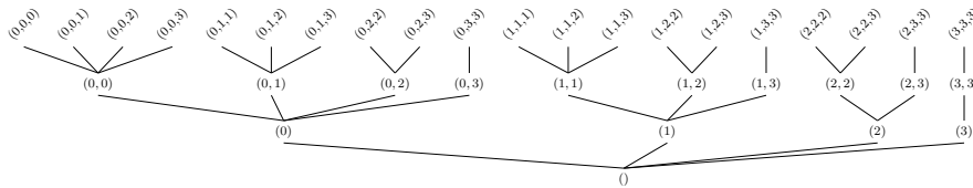
Figure 2: Initial structure of \omega^{\leq 3} .
