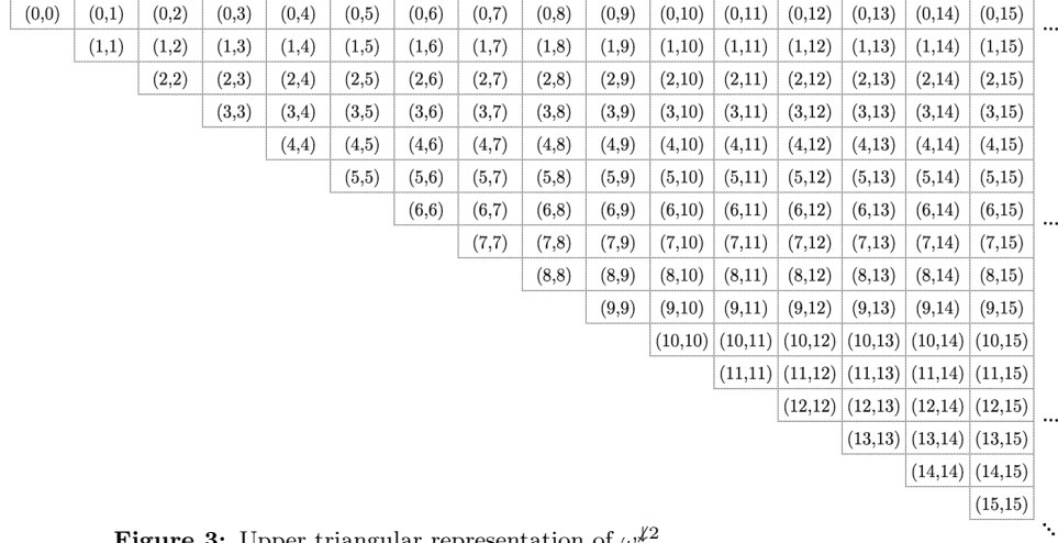
Figure 3: Upper triangular representation of \omega^{\mathbb{N}^2} .
