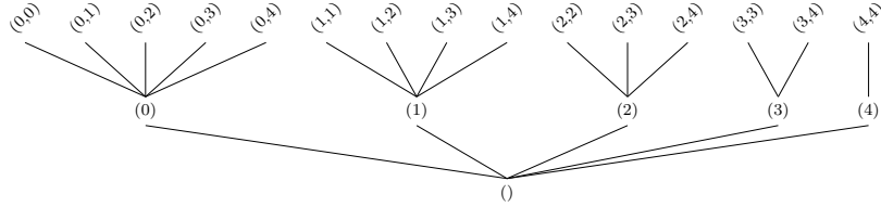
Figure 1: Initial structure of \omega^{\leq 2} .
