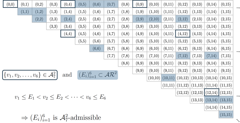
Figure 8: An \mathcal{A}_7^2 -admissible sequence.
