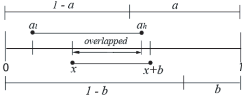
Figure 4: Join of two intervals
