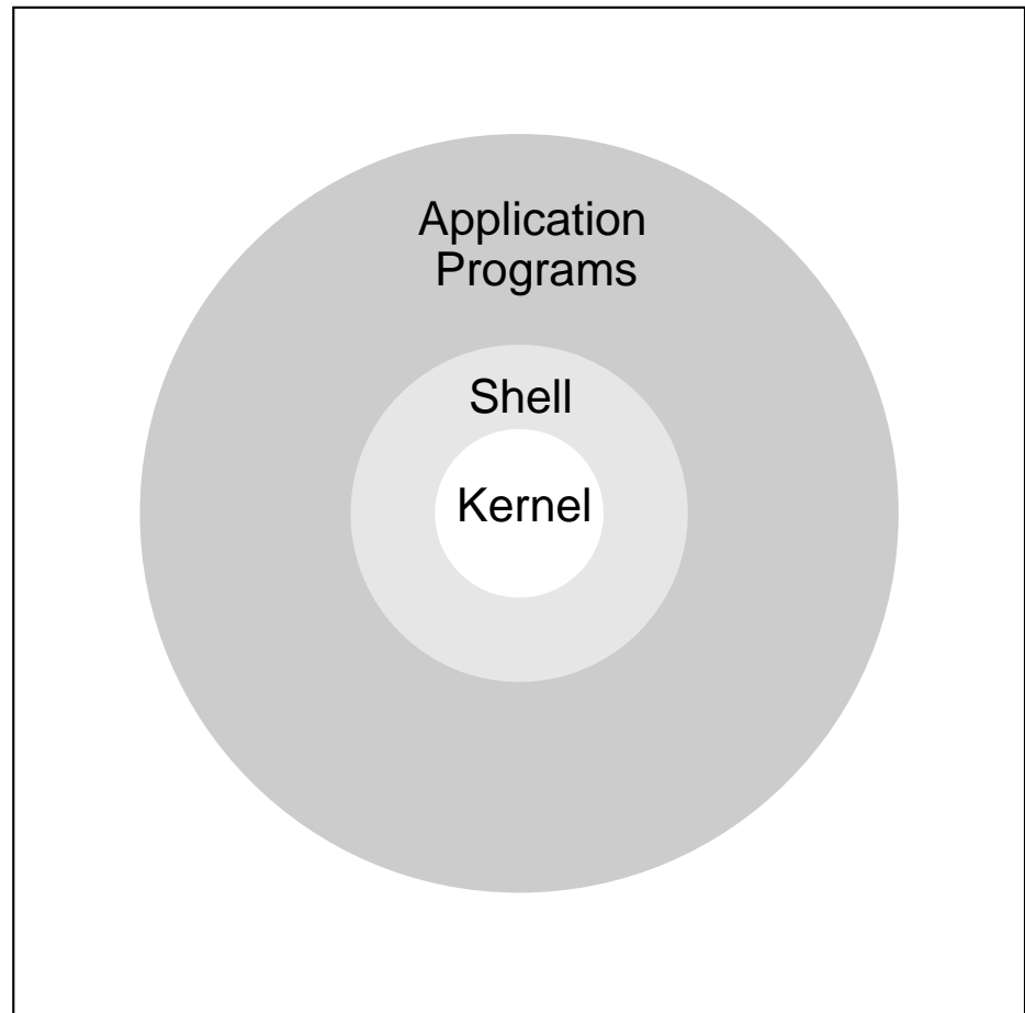
Figure 1.2: UNIX Systems
