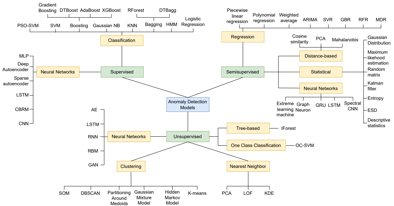
Fig. 6 Taxonomy of anomaly detection algorithms discussed in this work; Table A2 provides the list of works under a specific detection technique
